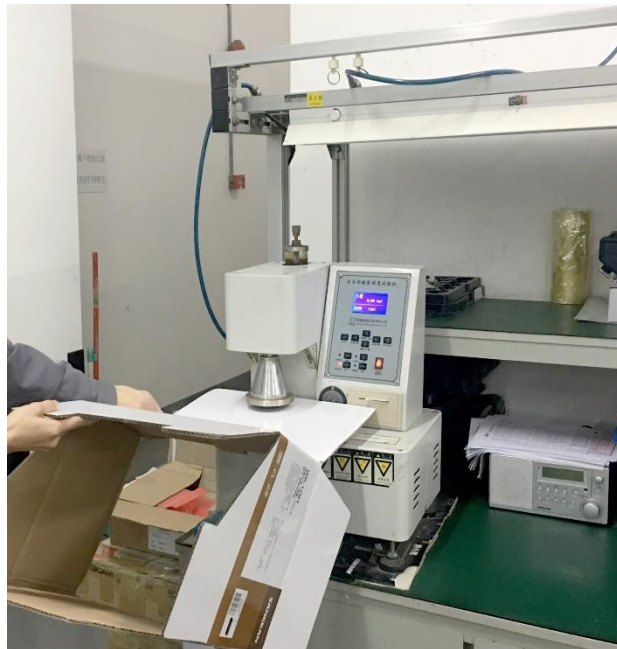
10 Carton Rupture Strength Testing Machine
